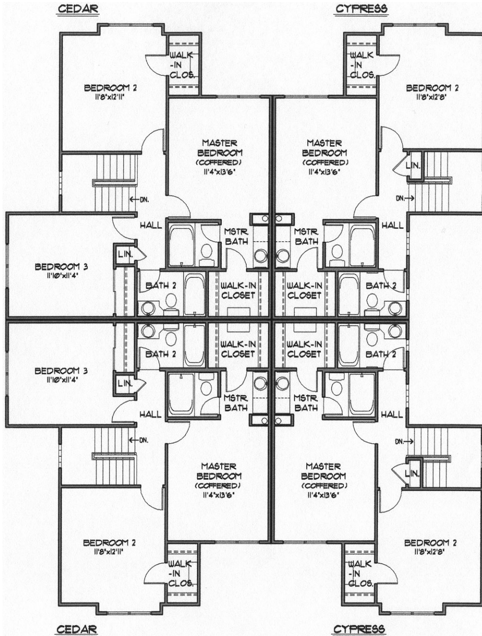
TOWNHOMES AT EMERALD GLEN UPPER LEVEL 4-PLEX COMPOSITE FLOOR PLAN
