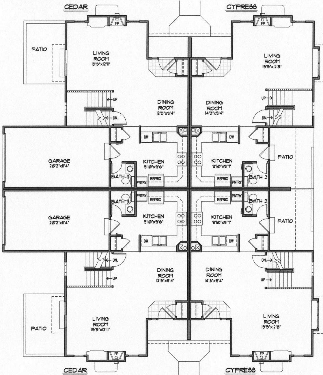
TOWNHOMES AT EMERALD GLEN MAIN LEVEL 4-PLEX COMPOSITE FLOOR PLAN
