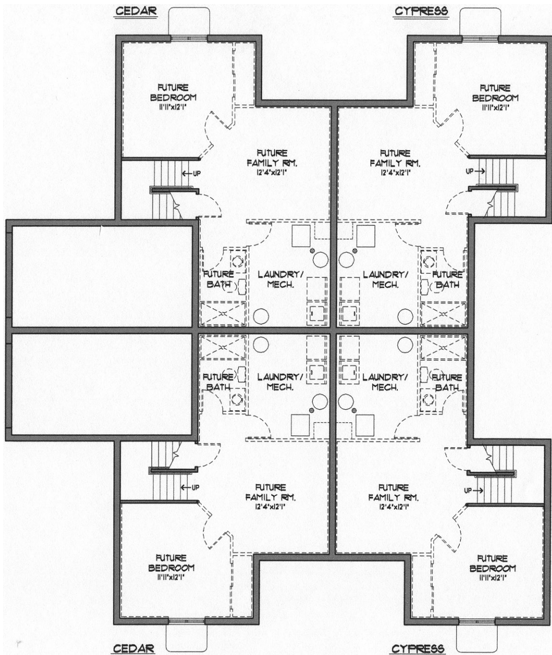
TOWNHOMES AT EMERALD GLEN BASEMENT LEVEL 4-PLEX COMPOSITE FLOOR PLAN
